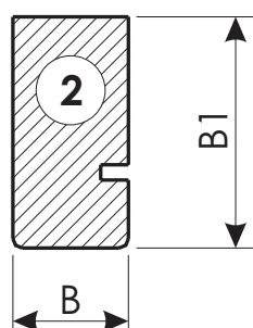
COPRIFILO COVER MOULD
